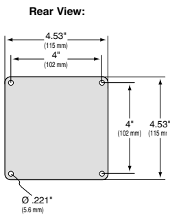
FX-30 Wall Mount Hole Pattern
